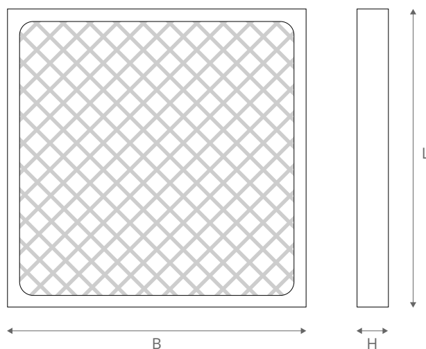
Model A, plantegning
